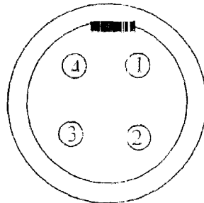
Pin out, viewed from solder end of panel mount socket
