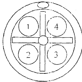
Pin out, viewed from solder end of plug
